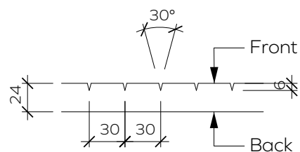
V-cut Detail
