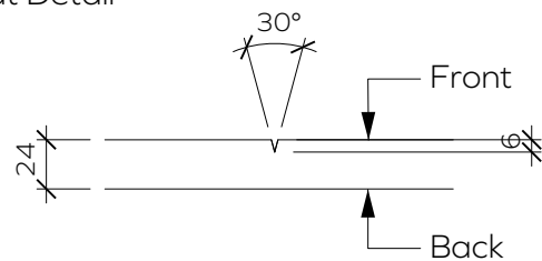
V-cut Detail
