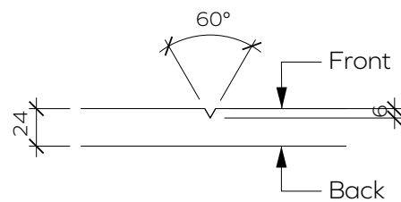
V-cut Detail
