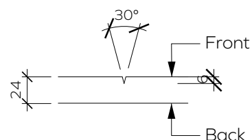
V-cut Detail
