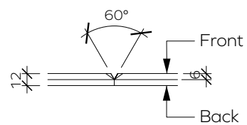
V-cut Detail
